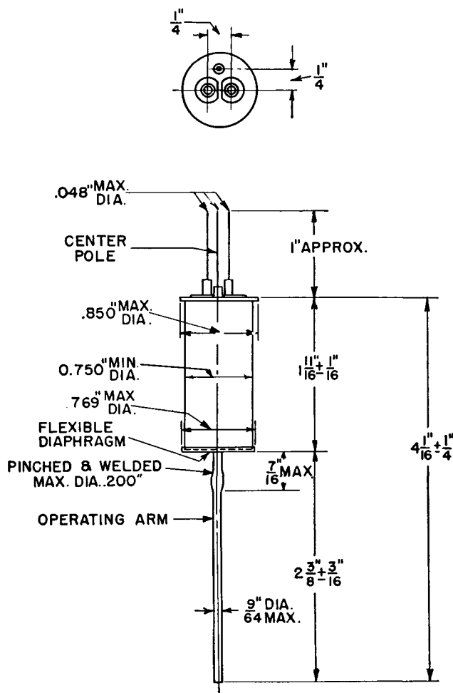
OUTLINE FA-6 VACUUM SWITCH
