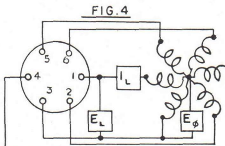
SIX-PHASE A.C. CONNECTION
