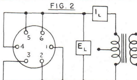
SINGLE-PHASE A.C. CONNECTION
