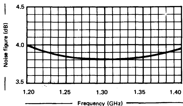
Noise figure
