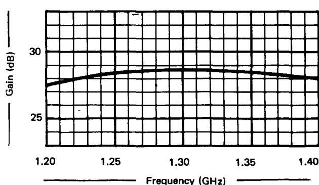
Gain
