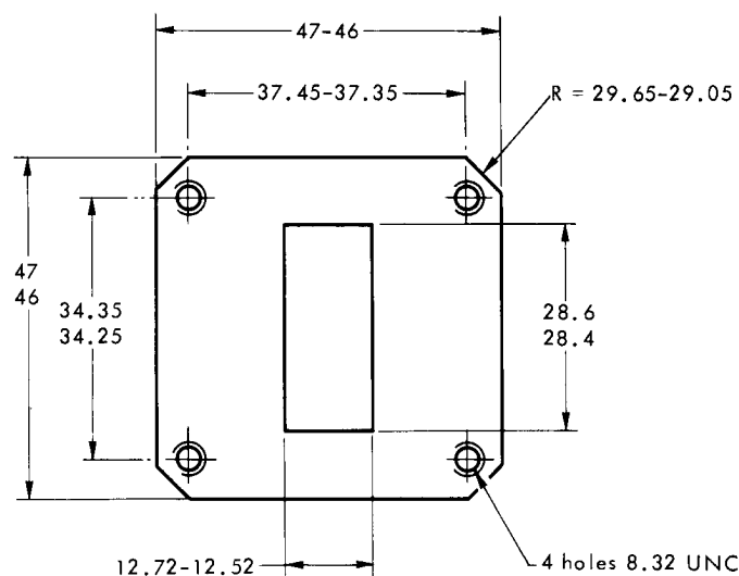
Output flange
