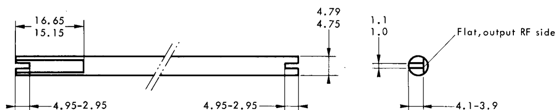
Detail, tuner shaft
