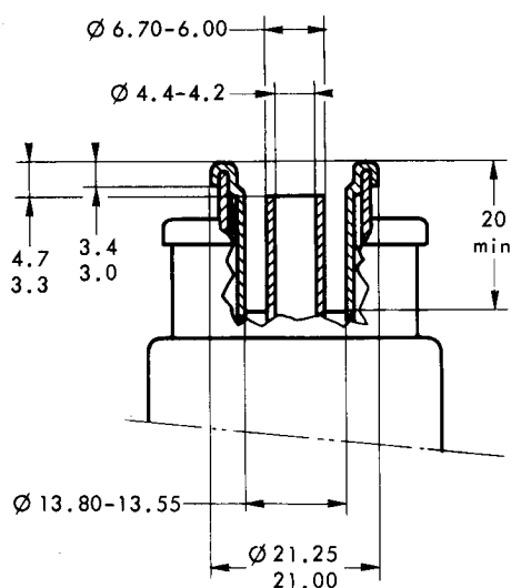
Detail, input connection
