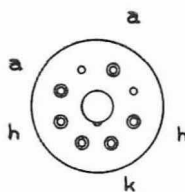
OCTAL BASE
