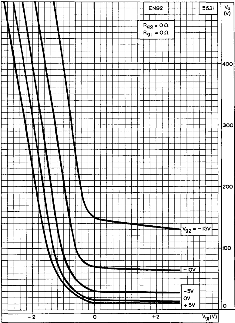
CONTROL CHARACTERISTICS
