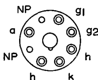
Octal Base
