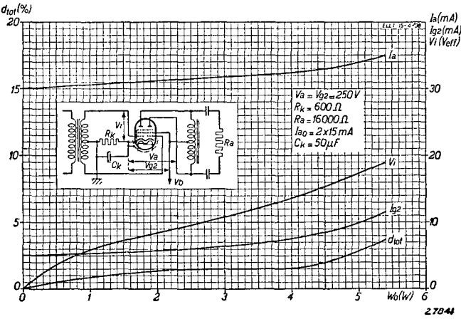
Fig. 5 Total distortion d_{\text{tot}} , alternating grid voltage V_i , total anode current I_a and total screen current I_{g2} , as functions of the output power of the ELL 1 when used in a balanced output stage with automatic grid bias.
