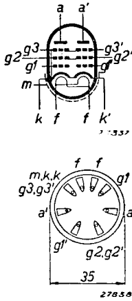
Fig. 2 Arrangement of electrodes and base connections.
