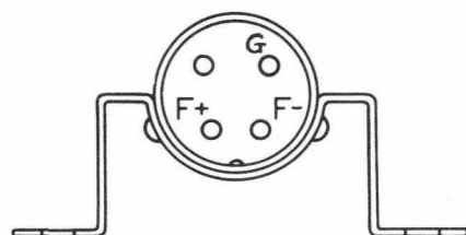
BOTTOM VIEW OF BASE
