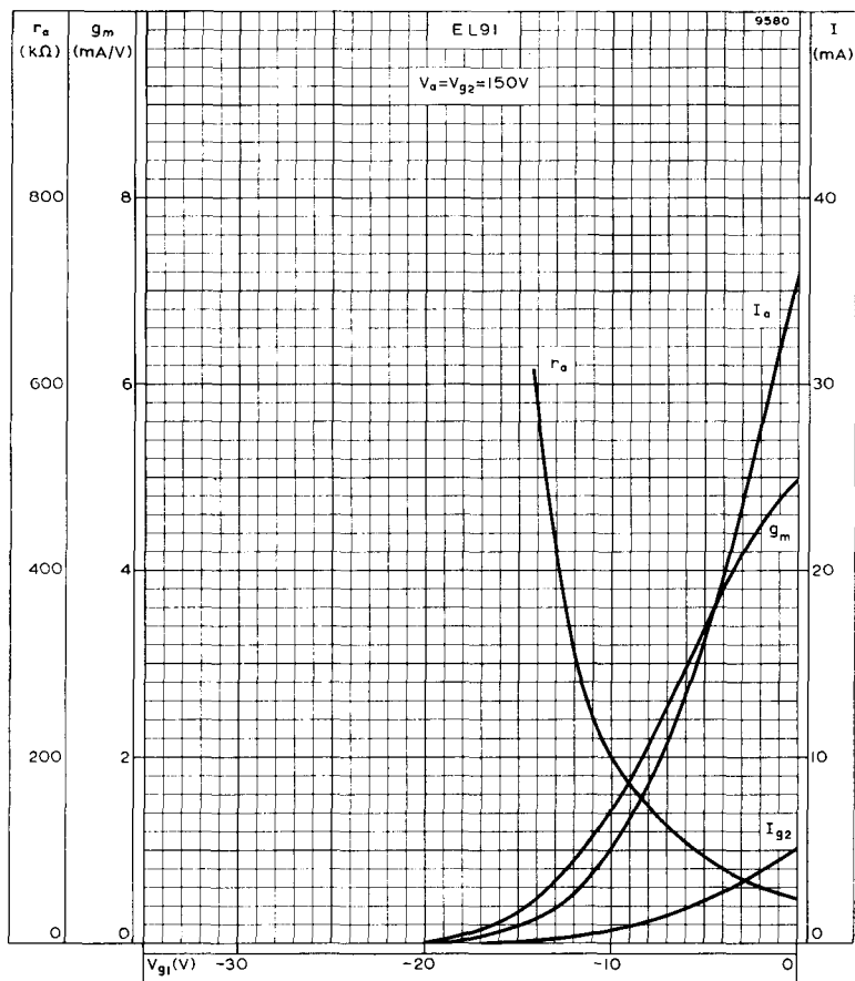
ANODE AND SCREEN-GRID CURRENTS, MUTUAL CONDUCTANCE AND ANODE IMPEDANCE PLOTTED AGAINST CONTROL-GRID VOLTAGE. V_{it} = V_{g2} = 150V
