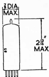
B9A Base
