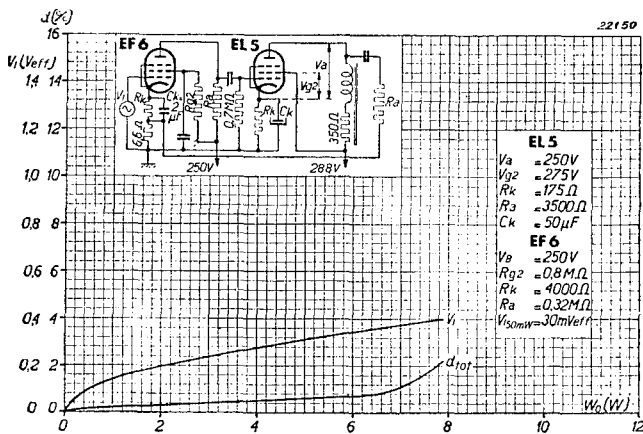
Fig. 7 Relation between alternating grid voltage V_i , total distortion d_{10t} and output power; EL 5 with pre-amplifier EF 6 and negative feedback applied to the latter.
