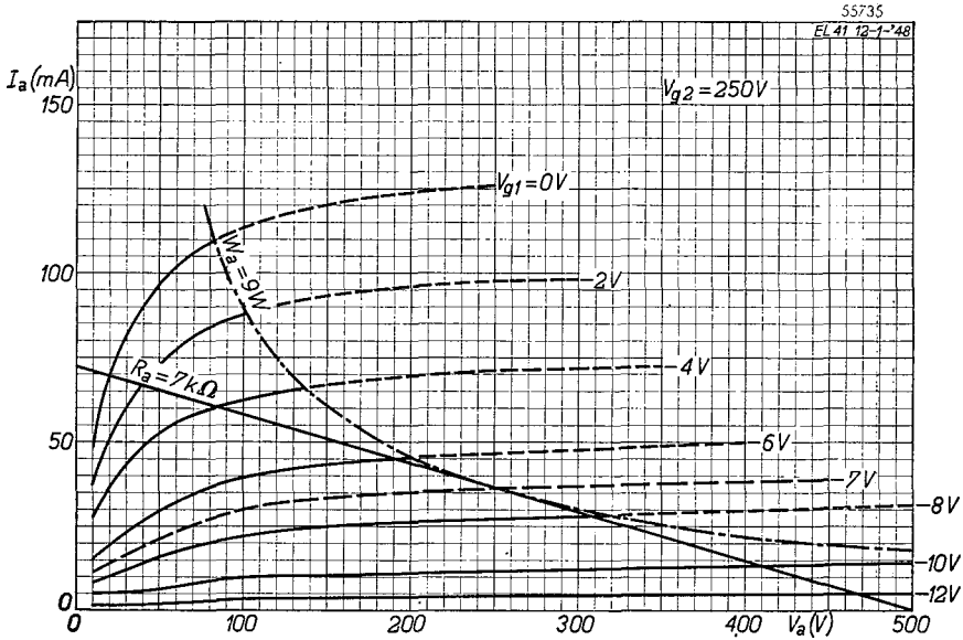
Anode current I_a as a function of the anode voltage V_a with the grid bias V_{g1} as parameter. Screen grid voltage V_{g2} = 250 V. The straight characteristic is the load line for an anode resistance R_a of 7\text{ k}\Omega . The dot-dash curve indicates the maximum permissible anode dissipation ( P_a = 9\text{ W} ).
