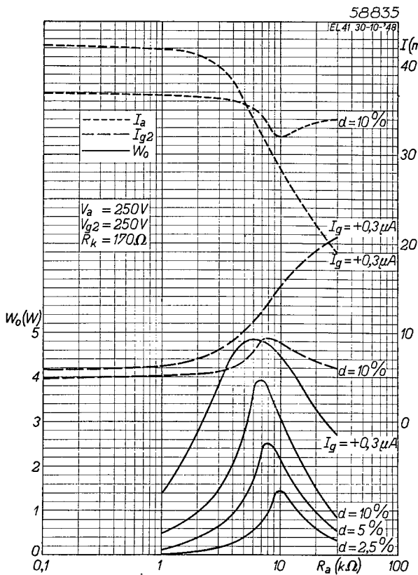
Fig. 10 Output power W_o of the EL 41 with 2\frac{1}{2} , 5 and 10% distortion and at the grid current starting point ( I_{g1} = +0,3\mu A ), as a function of the anode load resistance (continuous curves). Also the anode current I_a (dotted lines) and screen grid current I_{g2} (long dashes) with 10% distortion and at the grid current starting point ( I_{g1} = +0,3\mu A ), as function of the anode-load resistance R_a .
