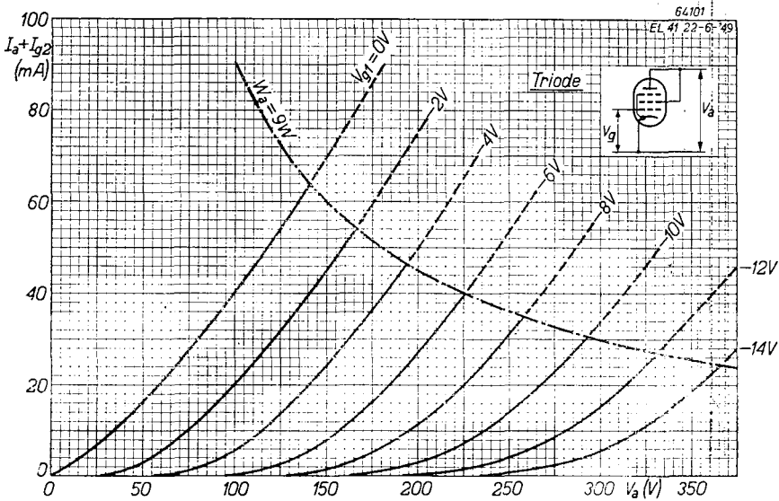
EL 41 connected as triode (screen grid connected to anode). Anode current I_a (including screen grid current) as function of the anode voltage. The dot-dash curve indicates the maximum per-
