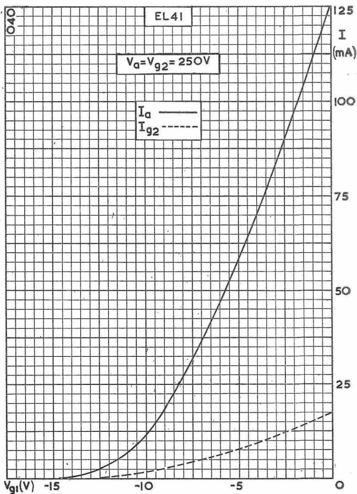
ANODE CURRENT AND SCREEN-GRID CURRENT PLOTTED AGAINST CONTROL-GRID VOLTS
