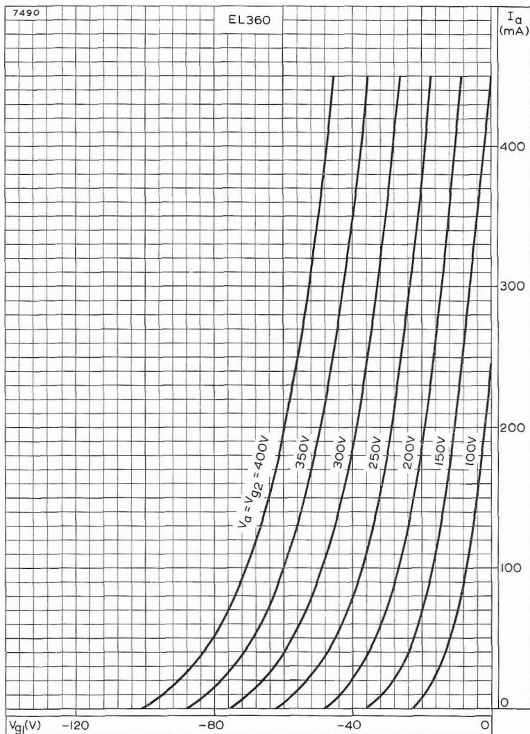
ANODE CURRENT PLOTTED AGAINST CONTROL-GRID VOLTAGE WITH ANODE AND SCREEN-GRID VOLTAGES AS PARAMETERS
