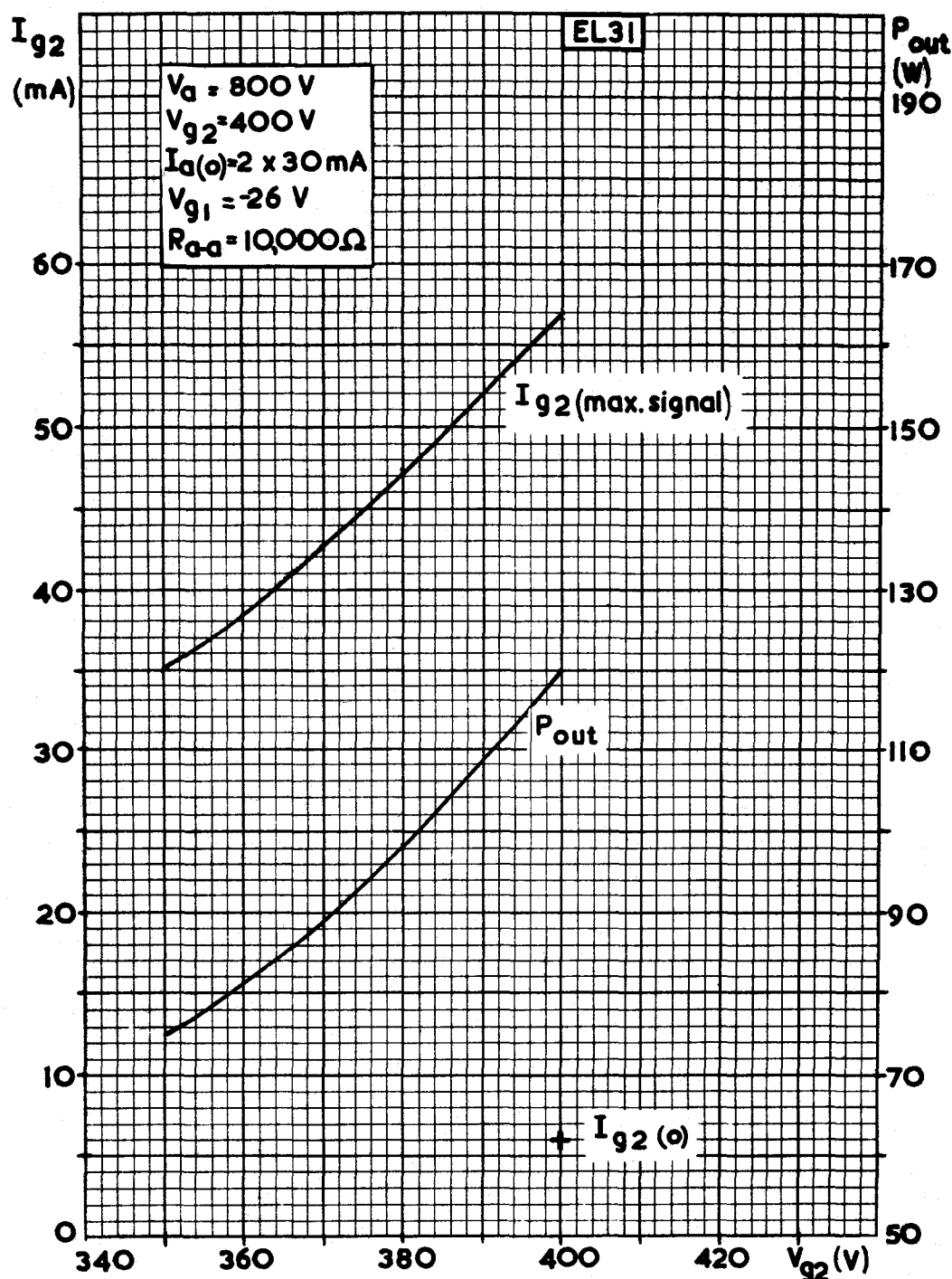
Fig. 22. Push-pull operating conditions with fixed bias and screen supply having poor regulation. ( V_{g2(b)} = 400 V. at V_a = 800 V).
