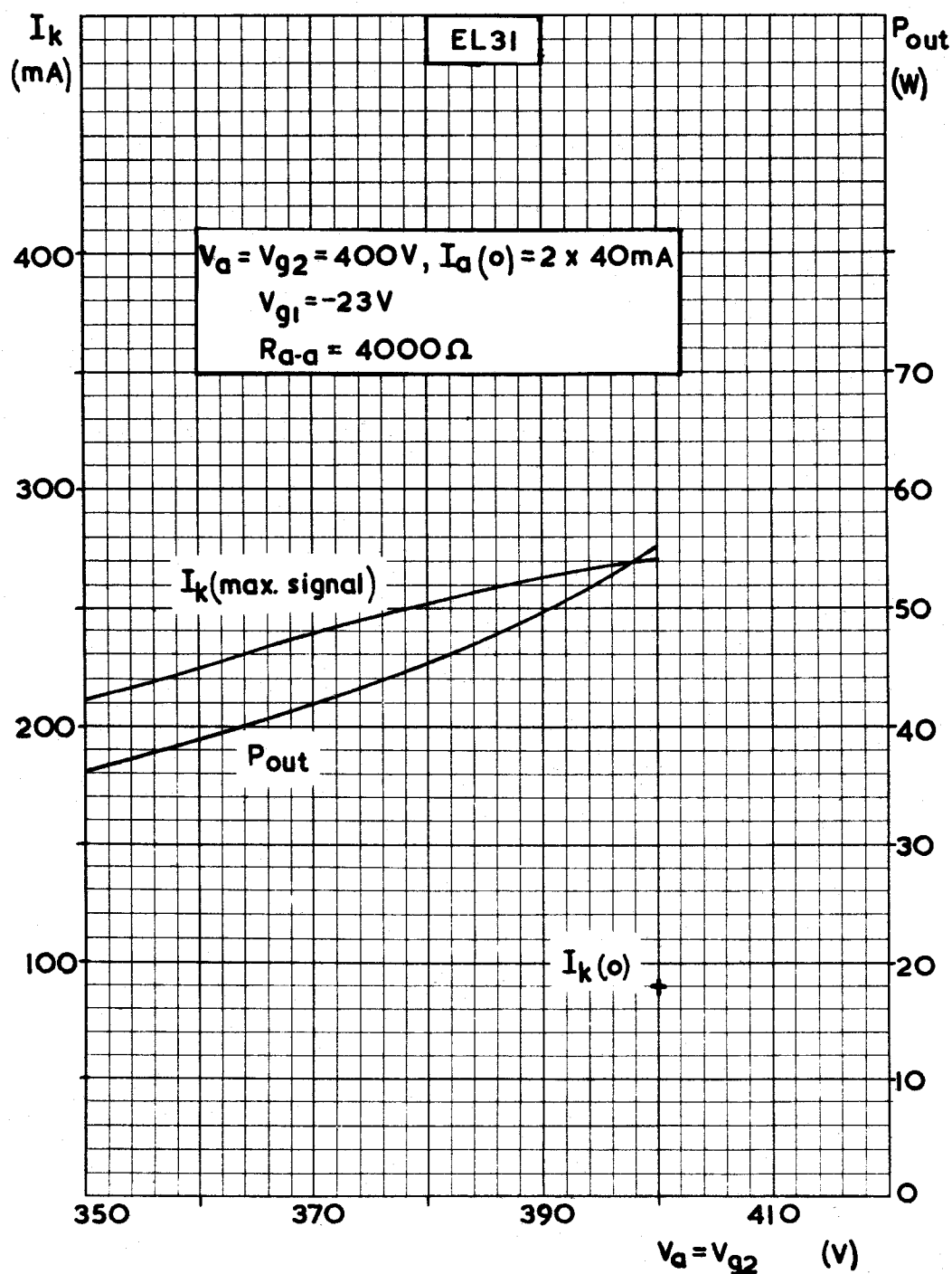
Fig. 16. Push-pull operating conditions with fixed bias and HT supply having poor regulation. ( V_b = 400 V ).
