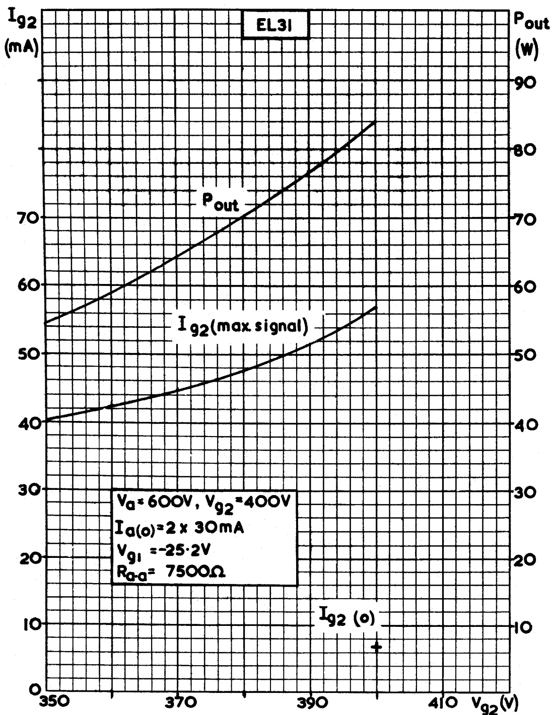
Fig. 19. Push-pull operating conditions with fixed bias and screen supply having poor regulation. ( V_{g2(b)} = 400\text{ V. at } V_a = 600\text{ V.} )
