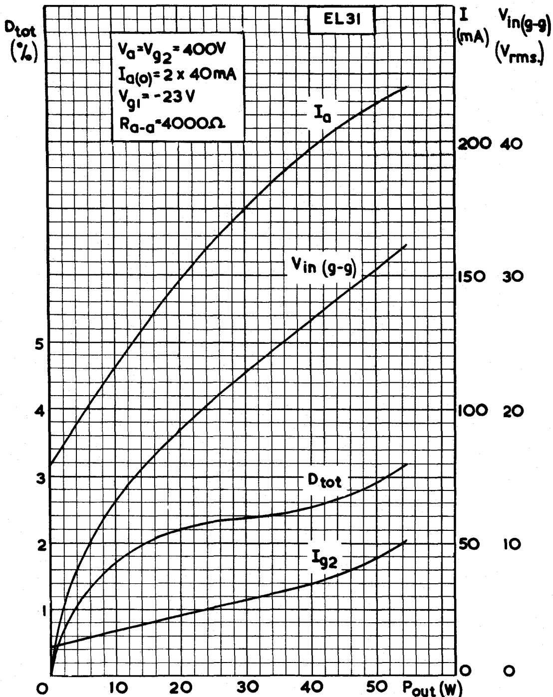
Fig. 15. Push-pull operating conditions for V_a = V_{g2} = 400V with fixed bias.
