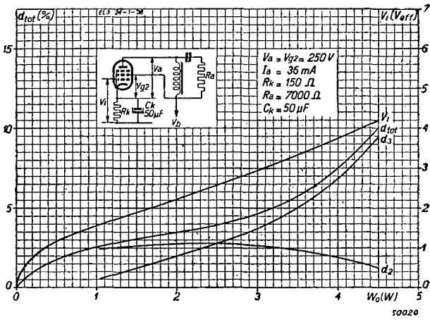
Fig. 6 Total distortion, 2nd and 3rd harmonic distortion and alternating grid voltage as a function of the output power. EL 3 used as single-output valve with automatic bias ( V_a = V_{g2} = 250 V ).
