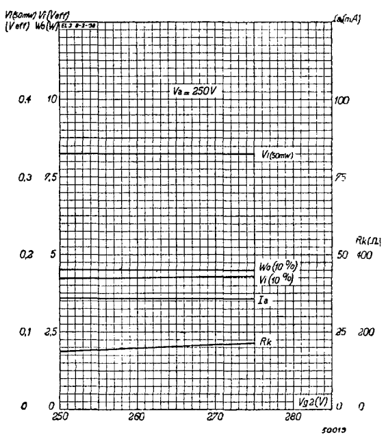
Fig. 7 Output power with 10 % distortion . . . W_o (10 %) Alternating grid voltage . . . V_i (10 %) Sensitivity . . . . . V_i (50 mW) Cathode resistor . . . . . R_k Anode current . . . . . I_a as a function of the screen-grid voltage (in the range 250–275 V), at constant anode voltage ( V_a = 250 V )
