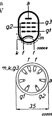
Fig. 2 Arrangement of electrodes and base connections.
