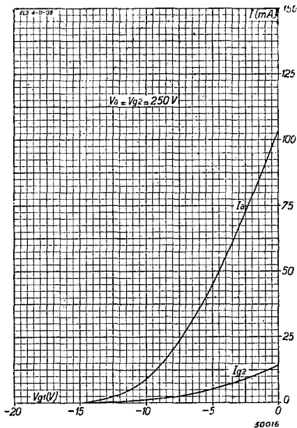
Fig. 4 Anode and screen-grid current as a function of the grid bias at V_a = V_{g2} = 250\text{ V} .
