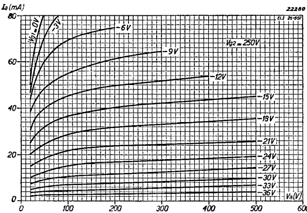
Fig. 4 Anode current as a function of the anode voltage with V_{g1} as parameter, at V_{g2} = 250 V.
