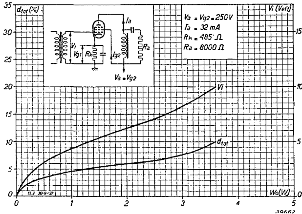
Fig. 8 Alternating grid voltage and total distortion as a function of the output power. EL 2 used as single output valve, with V_a = V_{g2} = 250 \text{ V} .
