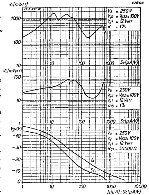
Fig. 7 Upper diagram. Alternating input voltage as a function of the conversion conductance controlled by the bias on grid 4, with 1% cross-modulation. Centre diagram. Alternating input voltage as a function of the conversion conductance controlled by the bias on grid 4, with 1% modulation hum. Lower diagram. Anode current and conversion conductance as a function of the bias on grid 4.
