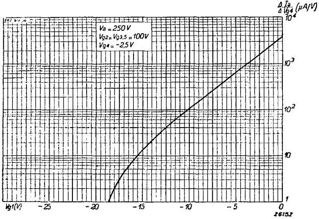
Fig. 5 Conversion of the 4th grid as a function of the direct voltage on grid 1
