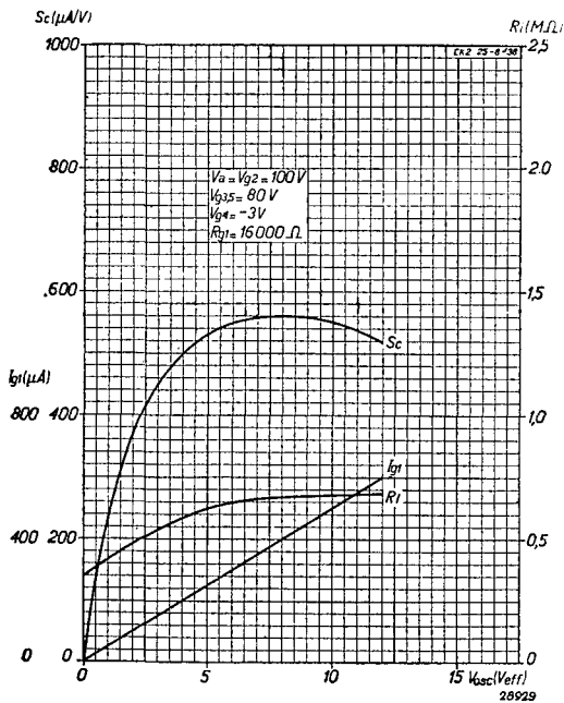
Fig. 6 Conversion conductance Sc , internal resistance Ri and oscillator-grid current I_{g1} as a function of the oscillator voltage, with V_{g2} = 100 V and V_{g3,5} = 80 V .
