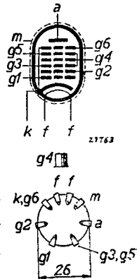
Fig. 2 Arrangement of electrodes and base connections.
