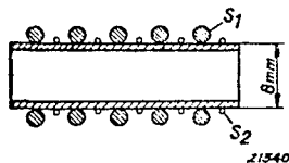
Fig. 14 Oscillator coil for use on very short waves (6 to 8 metres). S_1 = 5 turns of 2 mm bare copper wire (not tinned). S_2 = 5 turns of 0.1–0.2 mm enamelled copper wire.
