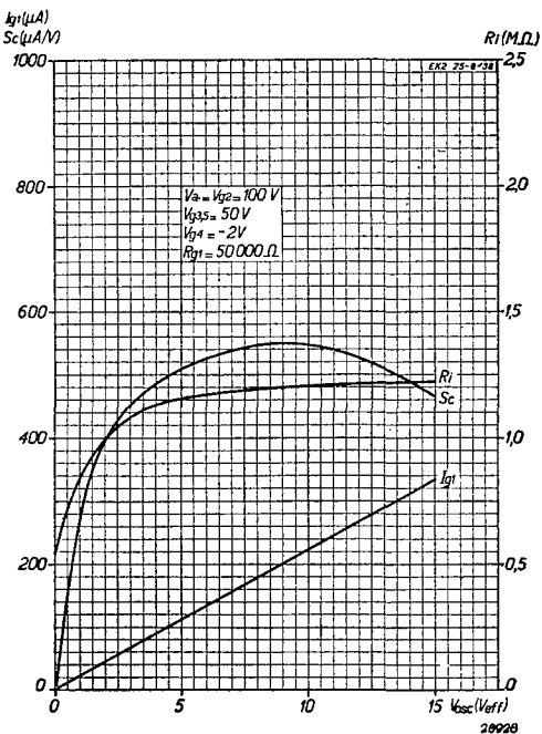
Fig. 7 Conversion conductance Sc , internal resistance Ri and oscillator-grid current I_{g1} as a function of the oscillator voltage, with V_{g2} = 100 V and V_{g3,5} = 50 V .
