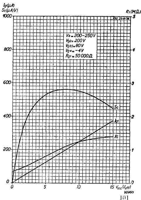
Fig. 5 Conversion conductance Sc , internal resistance Ri and oscillator-grid current I_{g1} as a function of the oscillator voltage, with V_{g2} = 200 V and V_{g3,5} = 80 V.
