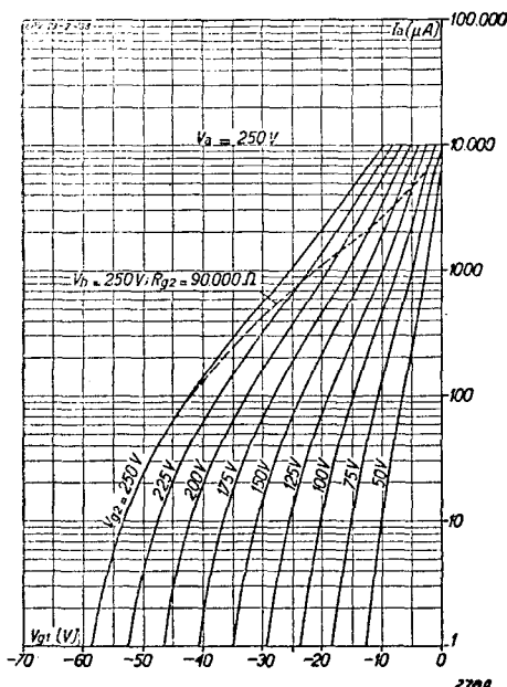
Fig. 3 I_a/V_{g1} characteristics using V_{g2} as parameter. The broken line shows the anode current with control applied to the valve, with the screen fed through a resistance of 90,000 ohms from a supply voltage of 250 V.
