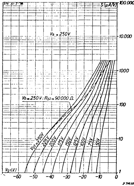
Fig. 4 Mutual conductance as a function of the grid bias, with V_{g2} as parameter. The broken line represents the mutual conductance of the valve when under control, with a screen-grid series resistor of 90,000 ohms and a supply voltage of 250 V.
