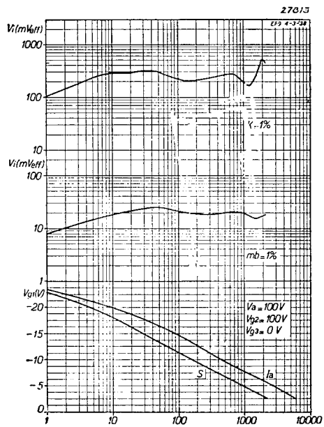
Fig. 8 Upper diagram. Effective alternating grid voltage as a function of the mutual conductance with 1 % cross-modulation, at V_a = 100 V, V_{g2} = 100 V (fixed). Centre diagram. Effective alternating grid voltage as a function of the mutual conductance with 1 % modulation hum. Lower diagram. Mutual conductance S and anode current I_a as a function of the grid bias.
