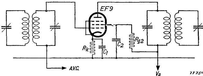
Fig. 5 Theoretical circuit diagram of an L.F. valve employing the principle of the "sliding" screen voltage.
