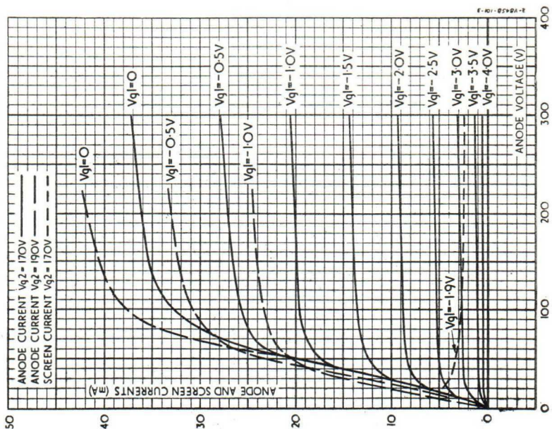
AVERAGE CHARACTERISTIC CURVES: I_a, I_g2/V_{g2}
