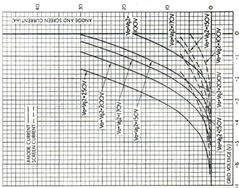
AVERAGE CHARACTERISTIC CURVES: I_a, I_g2/V_{g1}
