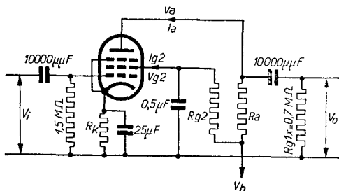
Fig. 9 Circuit diagram of the EF 6 employed as A. F. amplifier with resistance coupling.
