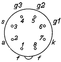
Fig. 2 Electrode arrangement, electrode connections and dimensions in mm of the EF 42.
