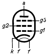
Fig. 2 Electrode arrangement, electrode connections and dimensions in mm of the EF 42.
