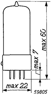
Fig. 2 Electrode arrangement, electrode connections and dimensions in mm of the EF 42.
