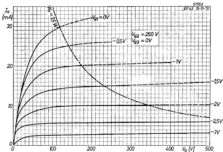
Fig. 5 I_a/V_a characteristics of the EF 42. The broken line indicates the maximum permissible anode dissipation ( W_a = 3.5 \text{ W} ).
