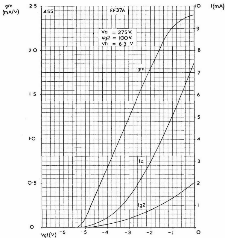
ANODE AND SCREEN-GRID CURRENTS AND MUTUAL CONDUCTANCE PLOTTED AGAINST CONTROL-GRID VOLTAGE. V_a = 275 V, V_{g2} = 100 V
