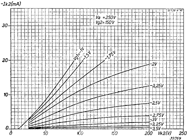
г. 14 Screen-grid current as a function of the secondary cathode voltage at different values of grid bias.
