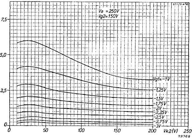
г. 14 Screen-grid current as a function of the secondary cathode voltage at different values of grid bias.
