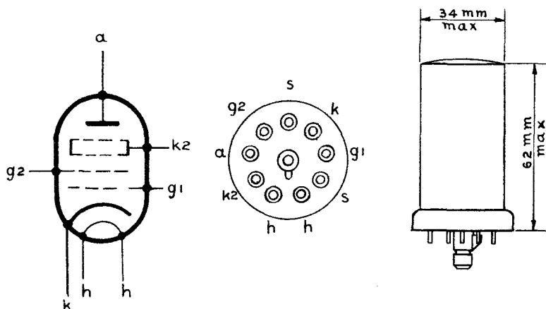
Arrangement of electrodes and base connections
