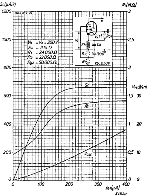
Fig. 10 Conversion conductance S_c , internal resistance R_i and alternating oscillator voltage V_{osc} as a function of the oscillator-grid current I_{g3} , at V_a = 250 V, R_{g3} = 50,000 ohms and with screen fed from a potential divider of 24,000 + 33,000 ohms (normal operation).
