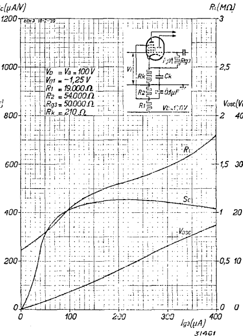
Fig. 14 Conversion conductance S_c , internal resistance R_i and alternating oscillator voltage V_{osc} as a function of the oscillator-grid current I_{g3} , at V_a = 100 V, R_{g3} = 50,000 ohms and with screen fed from a potential divider of 19,000 + 54,000 ohms (for receivers with switch for A. C. or D.C.).
