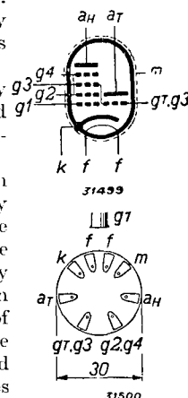
Fig. 2 Arrangement of electrodes and base connections.
