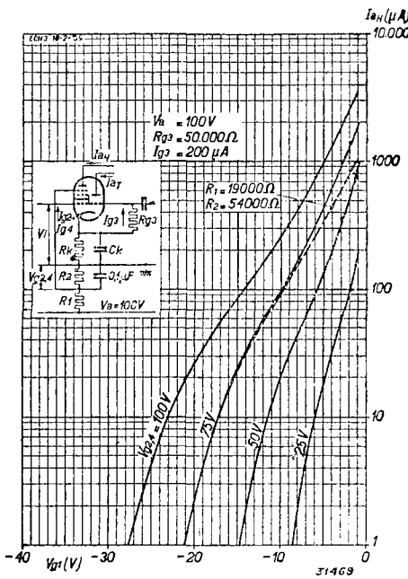
Fig. 6 Anode current of the hexode unit as a function of the grid bias, at different screen potentials, with an anode voltage of 100 V.
