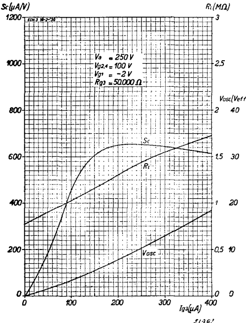
Fig. 9 Conversion conductance S_c , internal resistance R_i and alternating oscillator voltage V_{osc} as a function of the oscillator grid current I_{g3} , at V_a = 250 V, R_{g3} = 50,000 ohms and with fixed screen voltage of 100 V.
