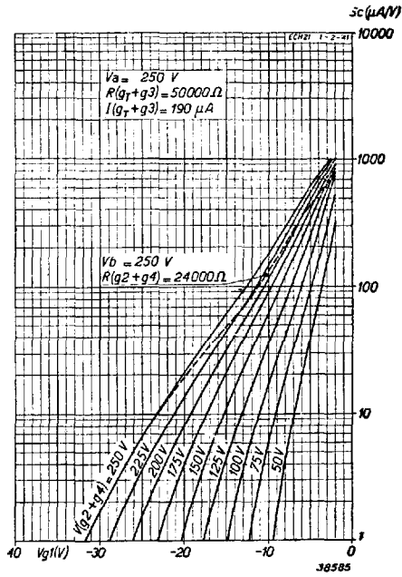
Fig. 9 Conversion conductance Sc as a function of grid bias V_{g1} , at an anode potential of 250 V, with screen voltage as parameter. The broken line refers to conditions for screen fed through a resistance of 24,000 Ohms.
