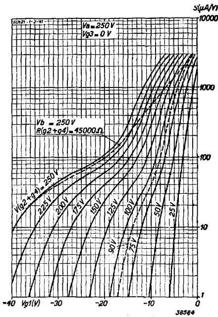
Fig. 13 Mutual conductance as a function of grid bias of the heptode section at V_a = 250 \text{ V} and V_{g3} = 0 \text{ V} , with screen voltage as parameter.
