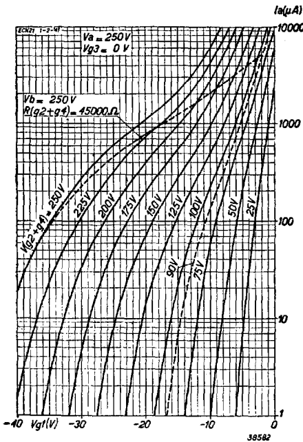
Fig. 12 The heptode section employed as I.F. amplifier. Anode current as a function of grid bias at V_a = 250 \text{ V} and V_{g3} = 0 \text{ V} with screen voltage as parameter.
