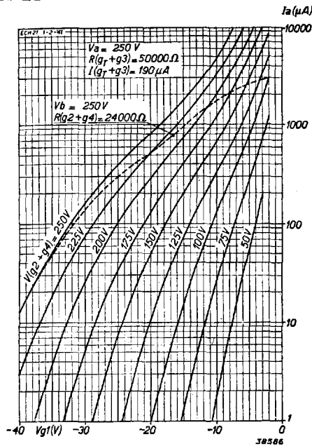
Fig. 8 Anode current of the heptode section as a function of grid bias, at an anode potential of 250 V, with screen voltage as parameter (valve used as frequency changer). The broken line refers to the conditions when the screen is fed across a resistance of 24,000 Ohms.
