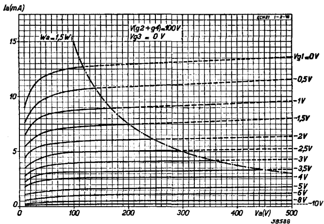
Fig. 15 Anode current as a function of anode voltage, with grid bias as parameter, at V(g_2 + g_4) = 100 V and V_{g3} = 0 V.
