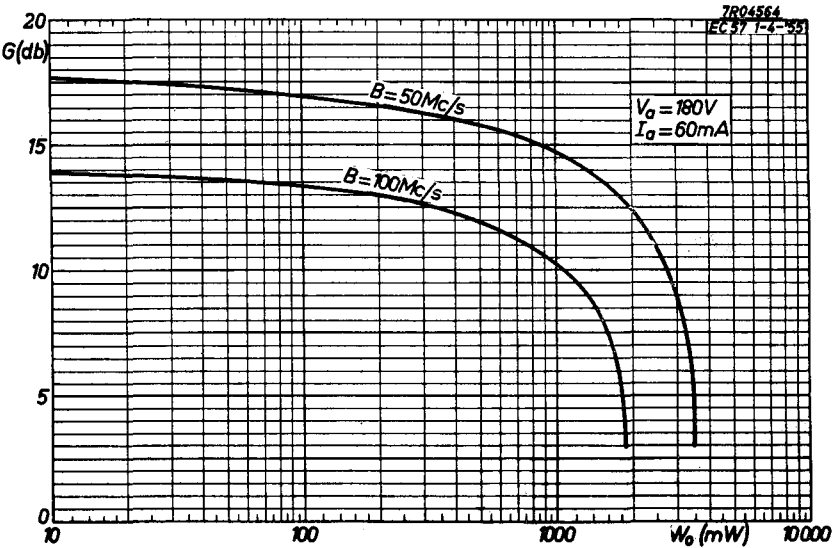
Fig. 48. Power gain G of the EC 57 as a function of the output power W_o with the bandwidth B as parameter at an anode current I_a = 60 \text{ mA} .
