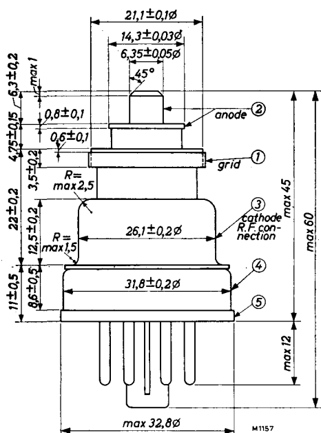
Fig. 40. Recommended mount*); dimensions in mm.
