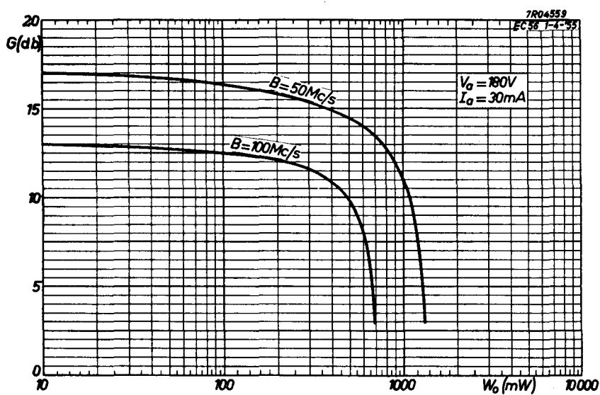
Fig. 46. Power gain G of the EC 56 as a function of the output power W_o with the bandwidth B as parameter at an anode current I_a = 30 \text{ mA} .
