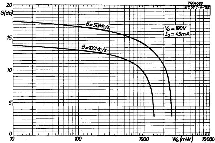
Fig. 47. Power gain G of the EC 57 as a function of the output power W_o with the bandwidth B as parameter at an anode current I_a = 45 \text{ mA} .
