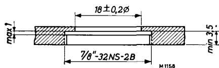
Fig. 40. Recommended mount*); dimensions in mm.
