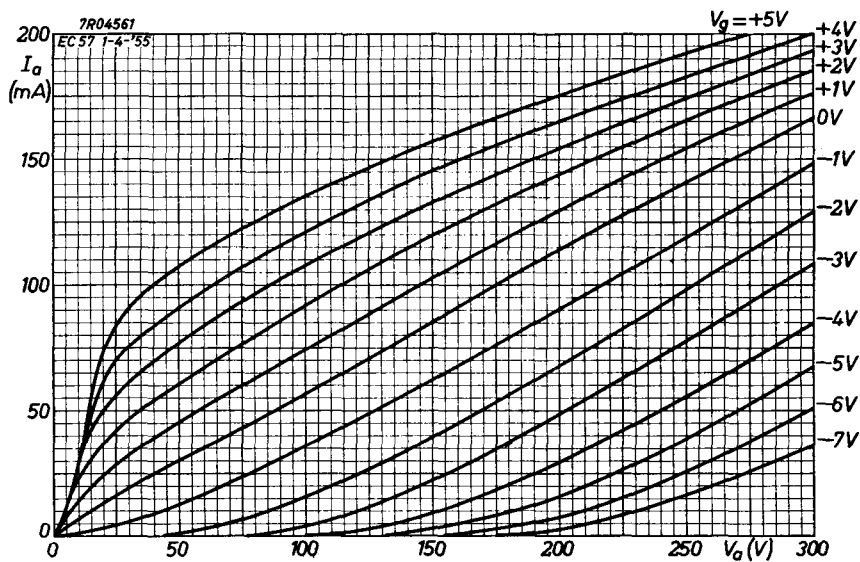
Fig. 44. I_a/V_a characteristics of the EC 57.
