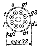
Fig. 3 Arrangement and connections of the electrodes.
