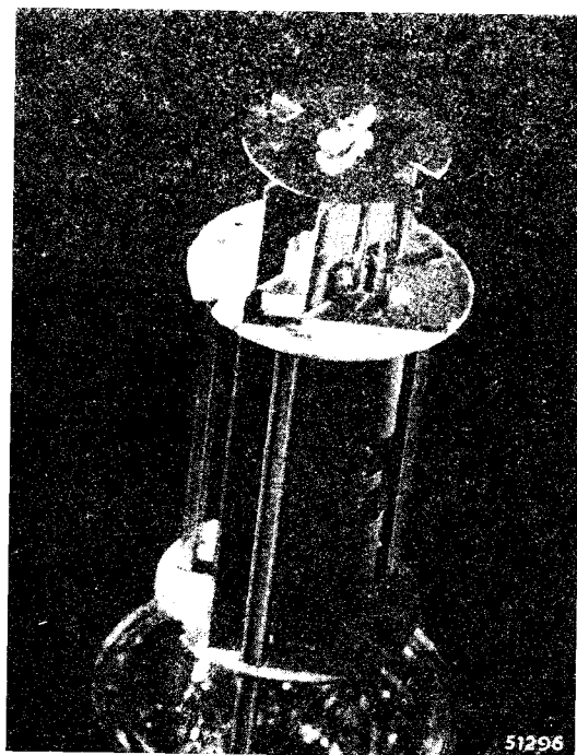
Fig. 1 Internal assembly of the double diode pentode EBL 21.
