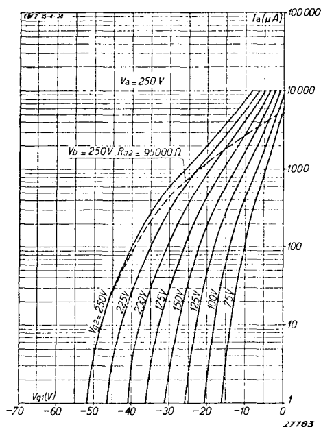
Fig. 3 I_a/V_{g1} characteristic of the EBF 2, with V_{a2} as parameter. The broken line shows the anode current of the controlled valve with a screen series resistor of 95000 ohms and a supply voltage of 250 V.
