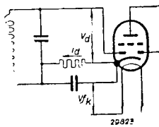
Fig. 5 Definition of V_d and I_d
