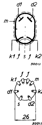
Fig. 2 Arrangement of electrodes and base connections.
