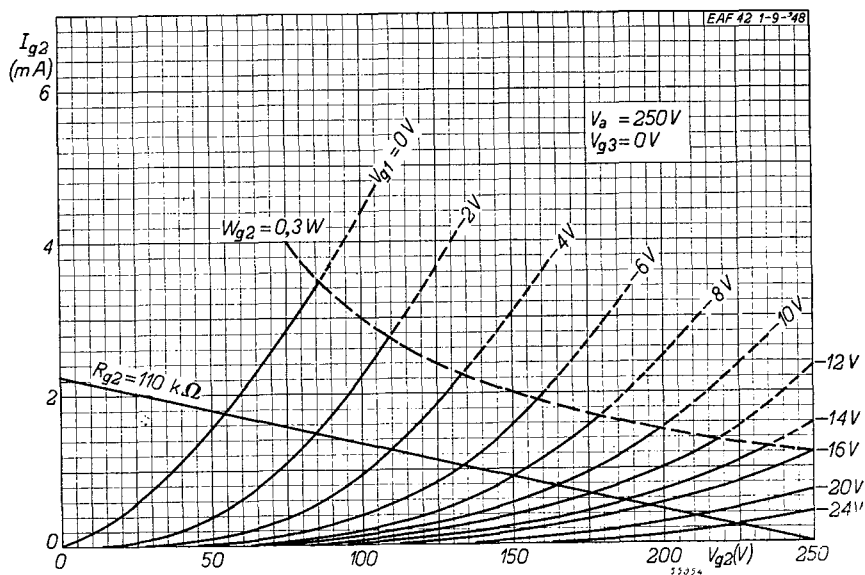
Fig. 17 Screen grid current ( I_{g2} ) of the pentode section of the ЕАФ 42 as a function of the screen grid voltage ( V_{g2} ), with grid bias ( V_{g1} ) as parameter. The broken line indicates the maximum screen grid dissipation (0.3 W). The straight line refers to a series resistor of 110 kΩ in the screen grid circuit (see Fig. 2).
