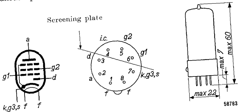
Fig. 7 Electrode arrangement, electrode connections and maximum dimensions in mm of the EAF 41. The screening plate, indicated by a line through the centre diagram, obviates undesirable coupling in the wiring. The letters i.c. at pin 4 indicate that this pin is internally connected to the electrode system and must not be connected to the external circuit.
