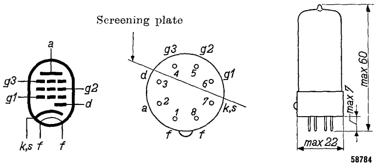
Fig. 8 Electrode arrangement, electrode connections and maximum dimensions in mm of the EAF 42. The screening plate shown in the centre diagram serves to reduce unwanted coupling in the wiring.
