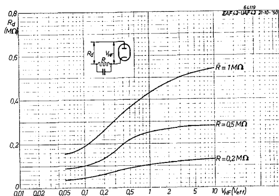
Fig. 16 Diode damping as a function of the applied R.F. voltage, for different values of the diode load resistance. This applies equally well to the diodes of the ЕАФ 41 and the ЕАФ 42.
