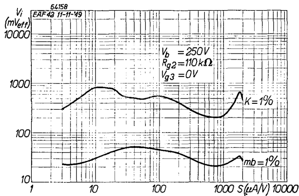
Fig. 15 R.M.S. voltage ( V_i ) of an interfering signal at the grid of the EAF 42, producing 1% cross modulation (curve K=1\% ), together with the R.M.S. value ( V_i ) of a hum voltage at the grid, resulting in 1% modulation hum (curve m_b=1\% ), measured as a function of the mutual conductance in the I.F. circuit shown in Fig. 2.
