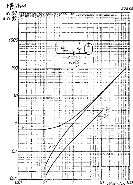
Fig. 3 Direct voltage V and direct voltage curve ( \Delta V ) between the terminals of the grid leak connected to one of the diodes of the EAB1, as a function of the unmodulated R.F. voltage. L.F. voltage V_{LF} between the terminals of the grid leak as a function of the R.F. voltage modulated to a depth of 30 % ( m = 30\% ). These characteristics apply to grid leaks of from 0.1 to 1 megohm.
