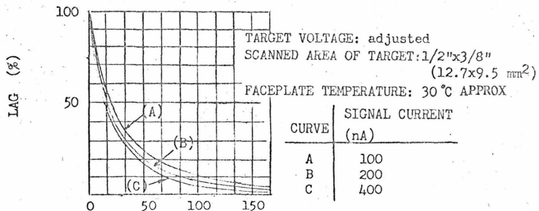
FIGURE 4. TYPICAL LAG CHARACTERISTICS
