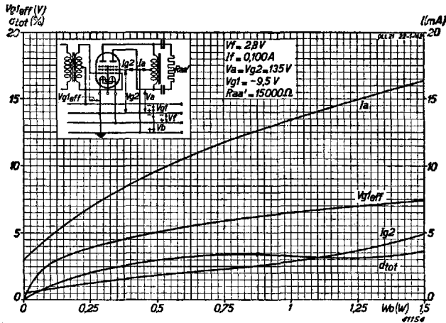
Fig. 19 Total anode current and screen grid current, total distortion and required alternating grid voltage per grid as function of output power at V_b = V_a = V_{g2} = 135 V, V_f = 2.8 V and I_f = 100 mA, in Class E circuit.
