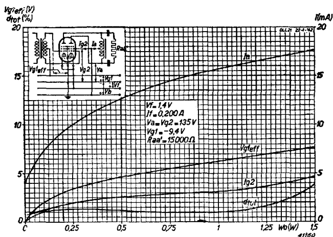
Fig. 13 Total anode current and screen grid current, total distortion and required alternating grid voltage per grid, as function of the output power at V_b = V_a = V_{g_2} = 135 V, V_f = 1.4 V, I_f = 200 mA in Class B circuit.
