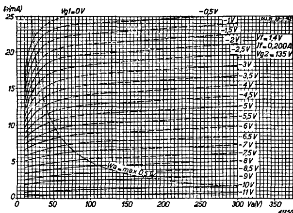
Fig. 12 Anode current of one pentode section as function of anode voltage at V_{g_2} = 135 V, V_f = 1.4 V and I_f = 200 mA, with V_{g_1} as parameter.
