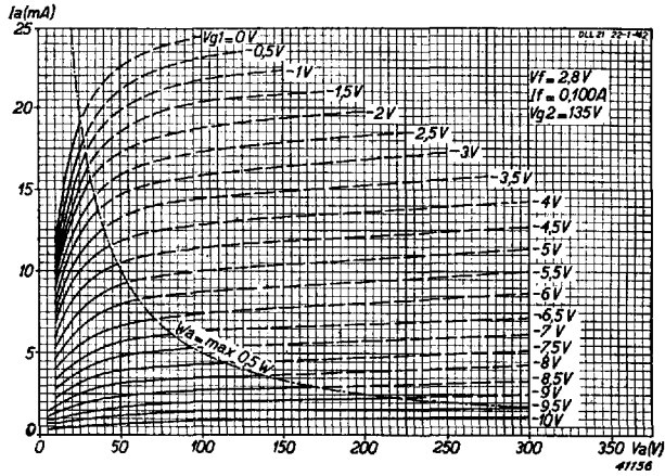
Fig. 18 Anode current of one pentode section as a function of anode voltage at V_{g2} = 135 V, V_f = 2.8 V and I_f = 100 mA, with V_{g1} as parameter.
