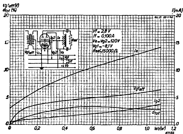
Fig. 17 Total anode current and screen grid current, total distortion and required alternating grid voltage per grid as function of output power, at V_b = V_a = V_{g2} = 120 V, V_f = 2.8 V and I_f = 100 mA, in Class B circuit.
