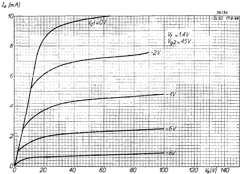
Fig. 4 Anode current ( I_a ) as a function of the anode voltage ( V_a ) with grid bias ( V_{g1} ) as parameter, at a screen grid voltage ( V_{g2} ) = 45\text{ V} . Filament connections 5 (—) and 1 + 7 (+), V_f = 1.4\text{ V} , I_f = 100\text{ mA} .
