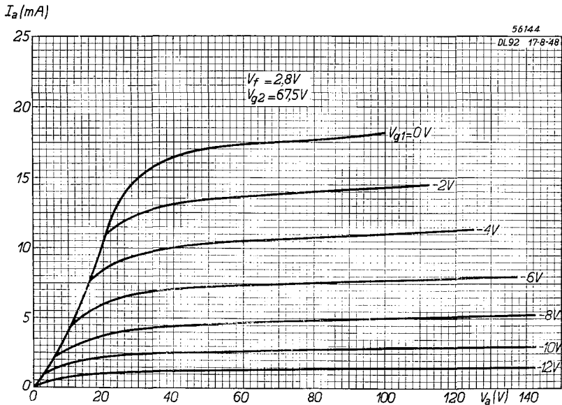
Fig. 14 I_a/V_a characteristics at V_{g2} = 67.5 V. Filament connections as for Fig. 13.
