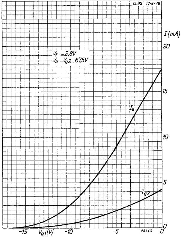
Fig. 13 Anode current ( I_a ) and screen grid current ( I_{g2} ) as functions of the grid bias ( V_{g1} ), at V_a = V_{g2} = 67.5 V. Filament connections 1 (—) and 7 (+), V_f = 2.8 V, I_f = 50 mA.
