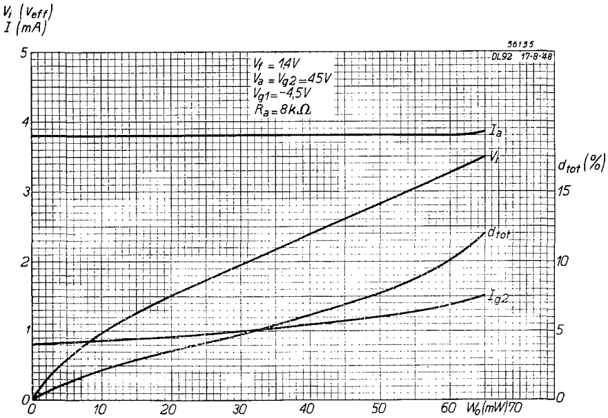
Fig. 5 Anode current ( I_a ), screen grid current ( I_{g2} ), required alternating input voltage ( V_i ) and distortion ( d_{tot} ) as functions of the output power ( W_0 ), at V_a = V_{g2} = 45\text{ V} . Filament connections as for Fig. 4.
