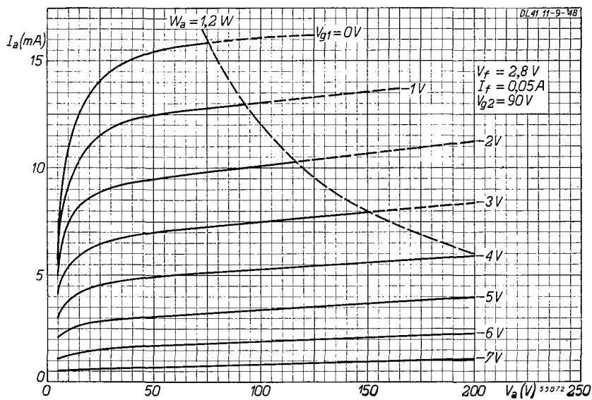
Fig. 14 I_a/V_a characteristics for a screen grid voltage of 90 V. Filament connections 7 and 8 ( V_f=2.8 \text{ V} , I_f=50 \text{ mA} ).
