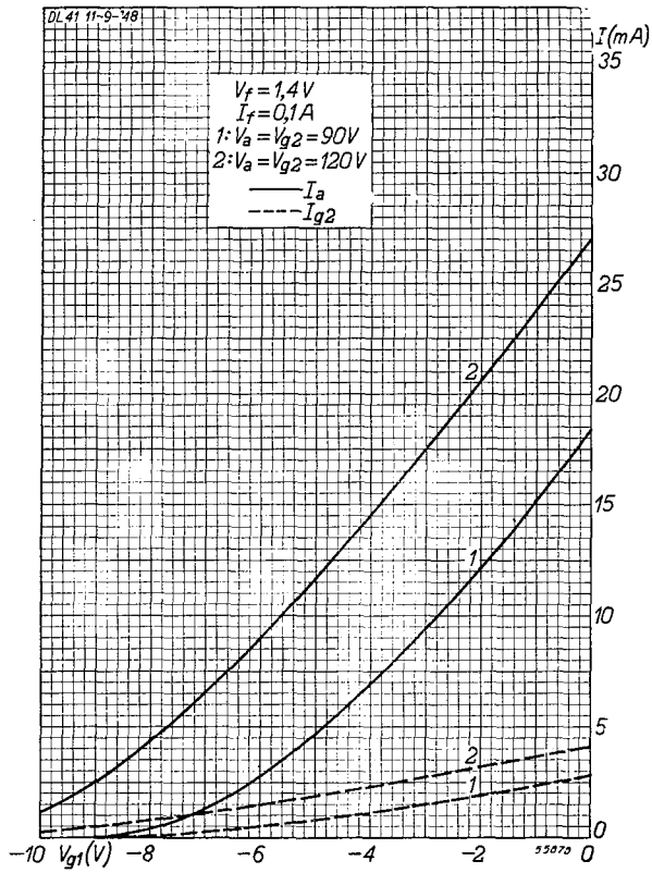
Fig. 8 Anode current ( I_a ) and screen grid current ( I_{g2} ) as functions of the grid bias ( V_{g1} ), with battery voltages of 90 and 120 V. Filament connections 1 and 7+8 ( V_f = 1.4 \text{ V} , I_f = 0.1 \text{ A} ).
