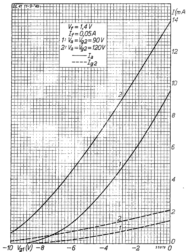
Fig. 3 Anode current ( I_a ) and screen grid current ( I_{g2} ) of the DL 41 as functions of the grid bias ( V_{g1} ), for battery voltages of 90 and 120 V. Filament connections 1 and 8 ( V_f = 1.4 \text{ V} , I_f = 50 \text{ mA} ).
