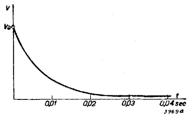
Fig. 10 Voltage on the grid of the output valve as a function of charging time of the grid condenser C in Fig. 9.
