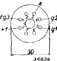
Fig. 2. Arrangement and sequence of contacts.
