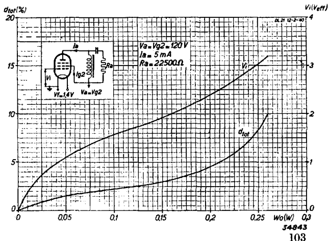
Fig. 5 Total distortion and required alternating grid voltage as function of output power at V_a = V_{g2} = 120 V.
