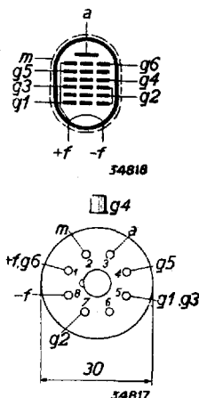
Fig. 2 Arrangement and sequence of contacts.
