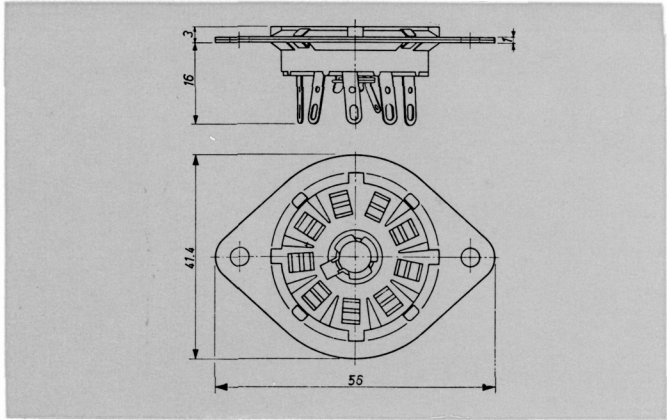
Base: English loctal 9 pins
