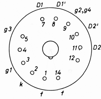
Base connections
