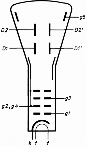
Electrode arrangement
