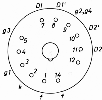
Base connections
