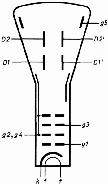
Electrode arrangement
