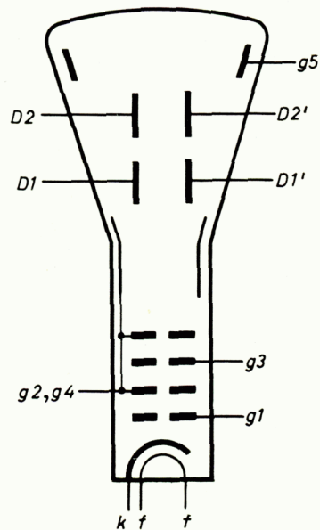
Electrode arrangement
