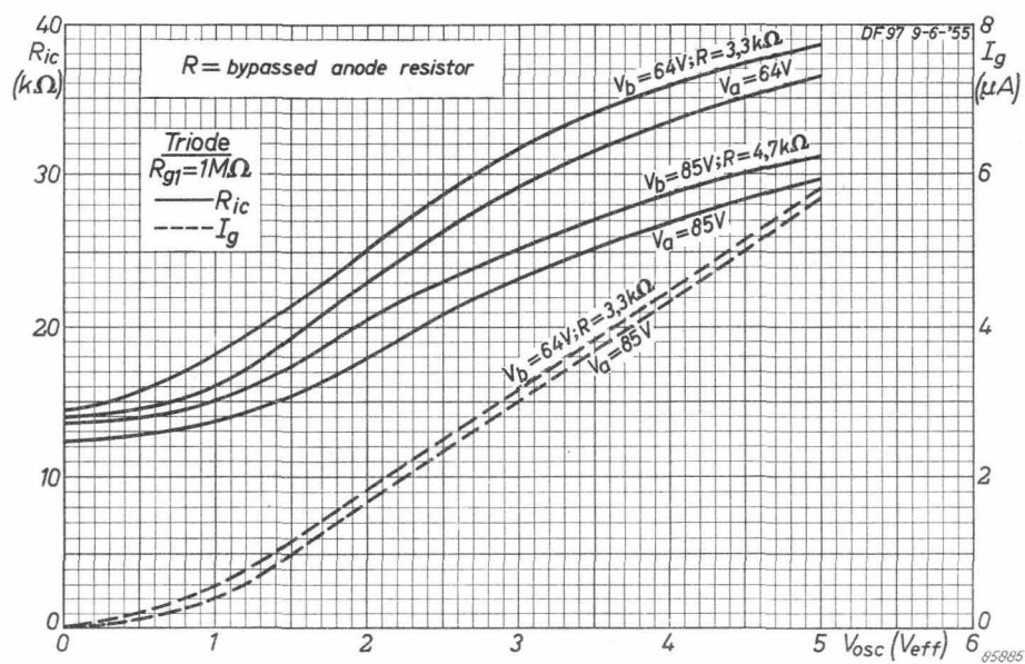
Fig.13. Grid current ( I_g ) and internal resistance ( R_{ic} ) as functions of the oscillator voltage V_{osc} ( V_{eff} ) at different values of the anode voltage V_a and the bypassed anode resistor R . Tube used as a self oscillating frequency changer in triode connection.
