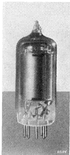
Fig. 1 The DF 91 (approximately full size).
