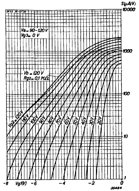
Fig. 4 Mutual conductance as a function of grid bias, at V_a = 90-120 V , with V_{g2} as parameter. The broken line refers to valve with control, the screen being fed from the 120 V source through a resistance of 0.1 M Ohm.
