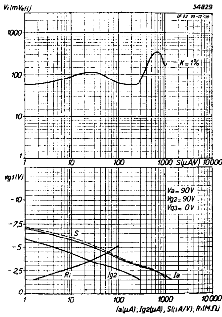
Fig. 8 Upper diagram; Effective value of alternating grid voltage as a function of mutual conductance, with 1 % cross modulation, at V_a = V_{g_2} = 90 V. Lower diagram; Mutual conductance S , anode current I_a , screen current I_{g_2} , and internal resistance R_i as a function of grid bias, at V_a = V_{g_2} = 90 V.
