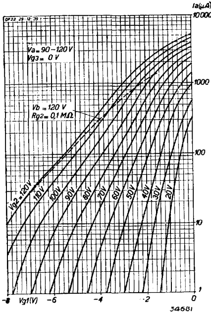
Fig. 3 Anode current as a function of grid bias, at V_a = 90-120 V , with V_{g2} as parameter. The broken line refers to a valve with control, the screen being fed from the 120 V source through a resistance of 0.1 M Ohm.
