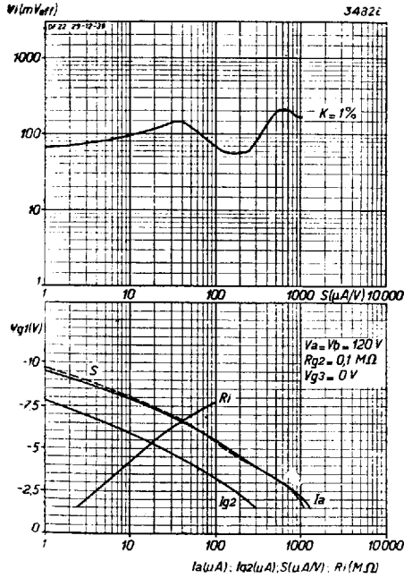
Fig. 7 Upper diagram; Effective value of alternating grid voltage as a function of mutual conductance, with 1 % cross modulation, at V_a = V_b = 120 V. Lower diagram; Mutual conductance S , anode current I_a , screen current I_{g_2} , and internal resistance R_i as a function of grid bias, at V_a = V_b = 120 V.
