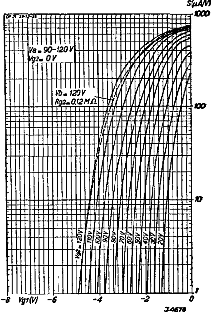
Fig. 5 Mutual conductance as a function of grid bias, at V_a = 90 - 120 V, with V_{g2} as parameter. The broken line represents the conditions for the controlled valve, with the screen fed from the 120 V source through a resistance of 0.12 M Ohm.
