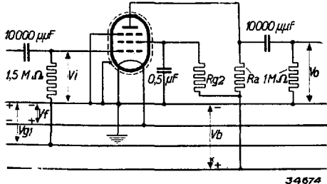
Fig. 3 Circuit diagram illustrating the symbols employed in the Operating Data
