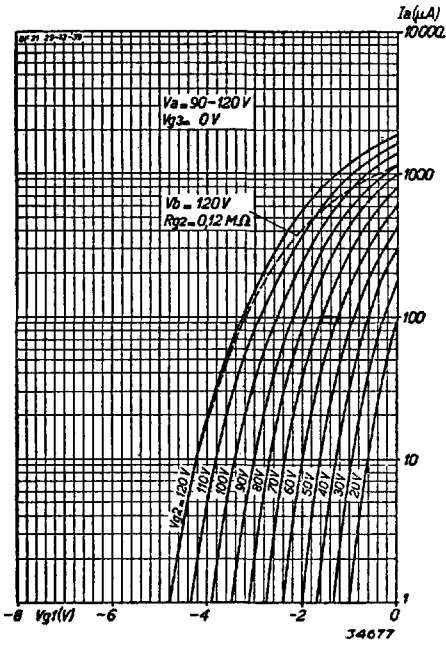
Fig. 4 Anode current as a function of grid bias at V_a = 90 - 120 V, with V_{g2} as parameter. The broken line represents the conditions for the controlled valve, with the screen fed from the 120 V source through a resistance of 0.12 M Ohm.
